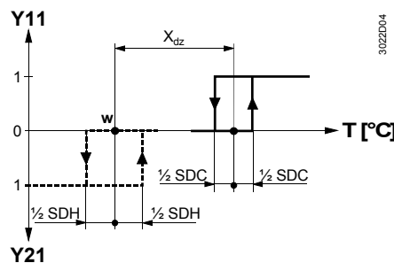
Cooling mode with optional electric heating sequence (DIP switch no.8 = ON)
