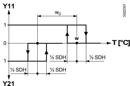
Heating mode (hot water plus electric)
